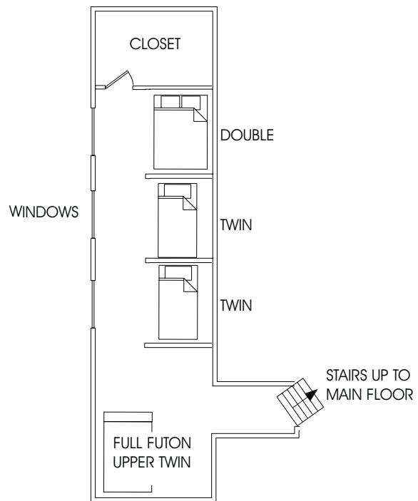
BUNKROOM FLOOR PLAN
